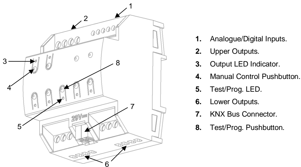
Figure 1. Elements scheme.
